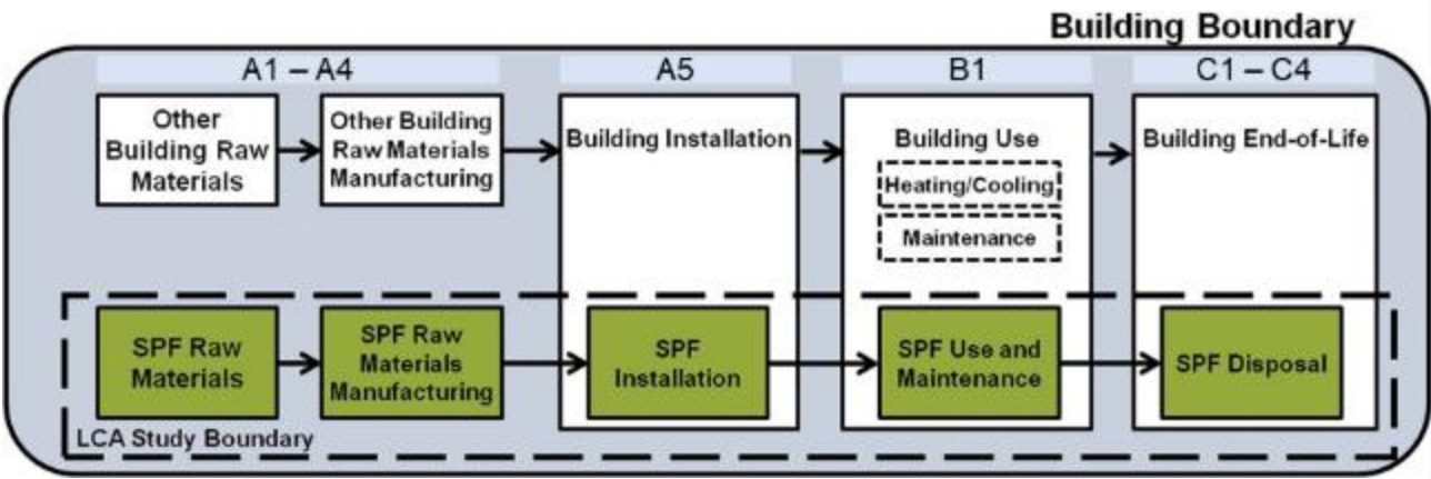
FIGURE 1 FLOW DIAGRAM OF SPRAY FOAM LIFE CYCLE
